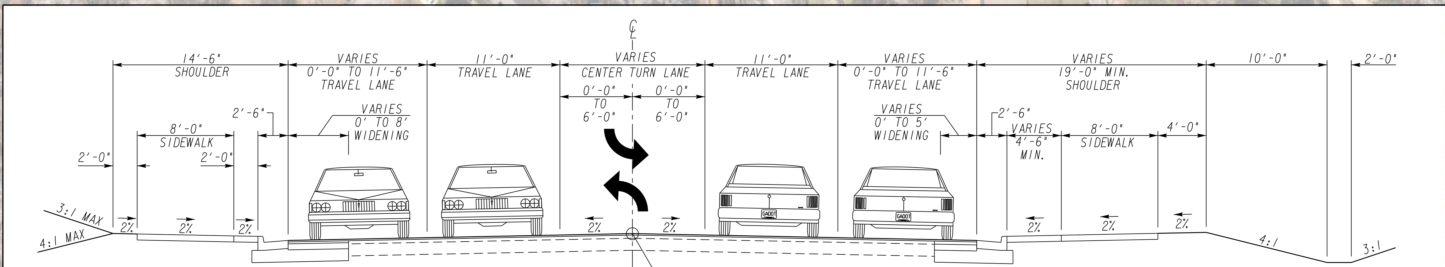
SR 154/SR 166/CAMPBELLTON ROAD URBAN 4-LANE - 12' FLUSH MEDIAN
