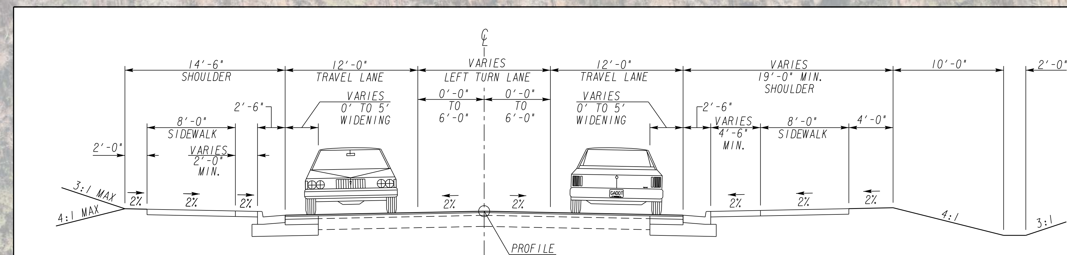
SR 154/SR 166/CAMPBELLTON ROAD URBAN 2-LANE
