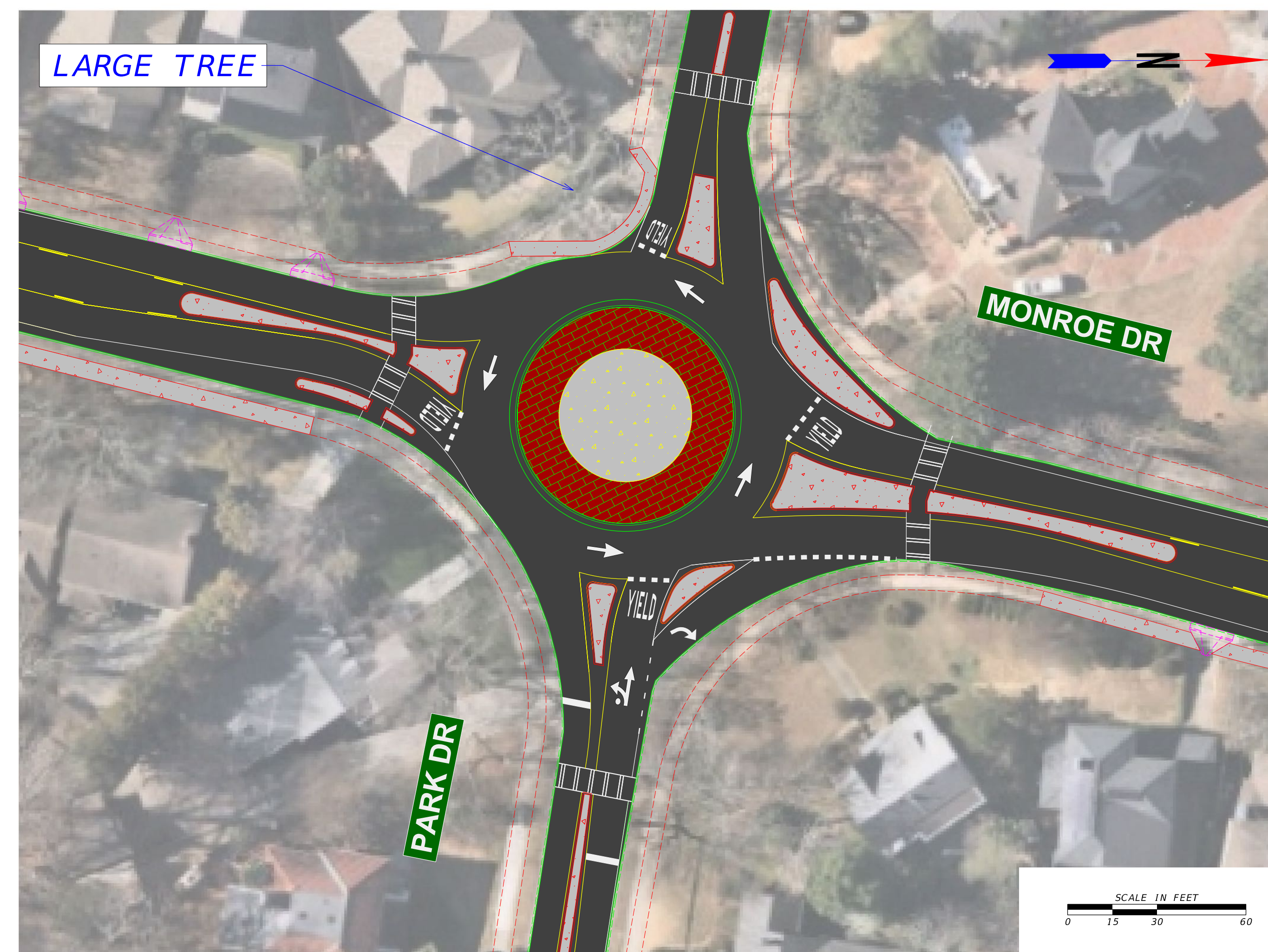
PARK DR ROUNDABOUT
