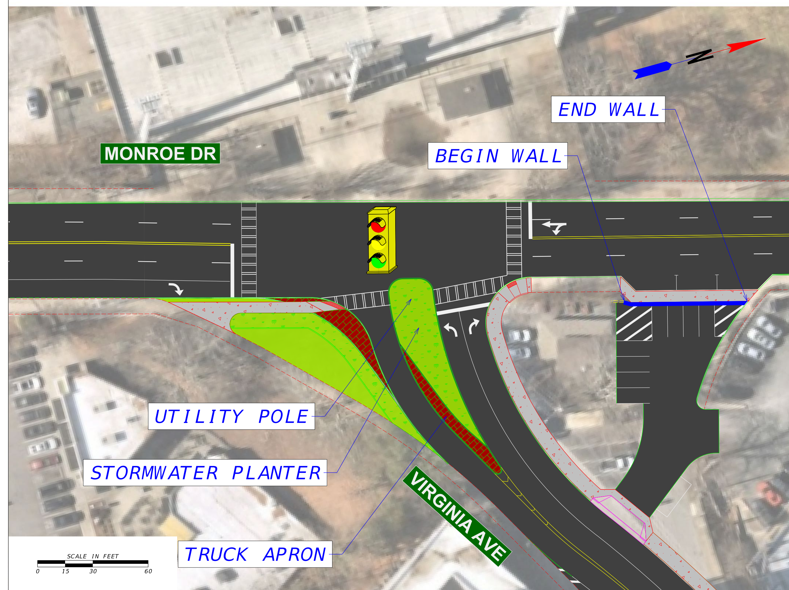
VIRGINIA AVE REALIGNMENT
