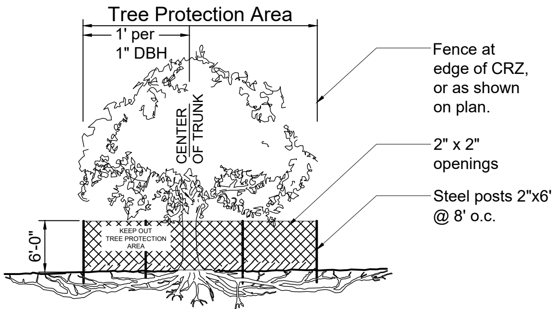
SECTION VIEW
