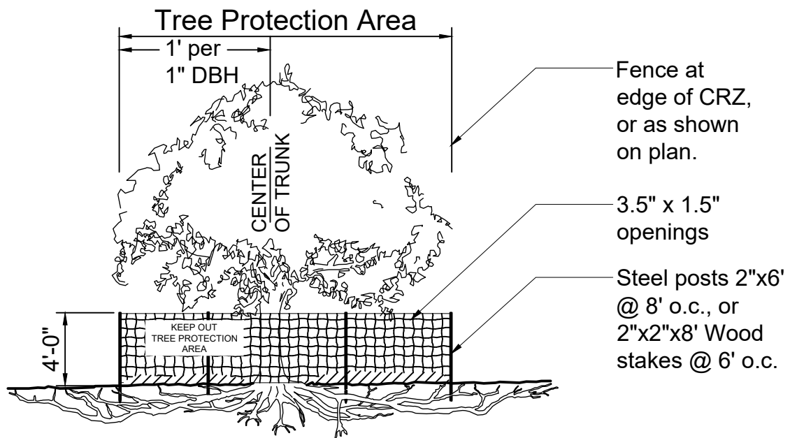
SECTION VIEW
